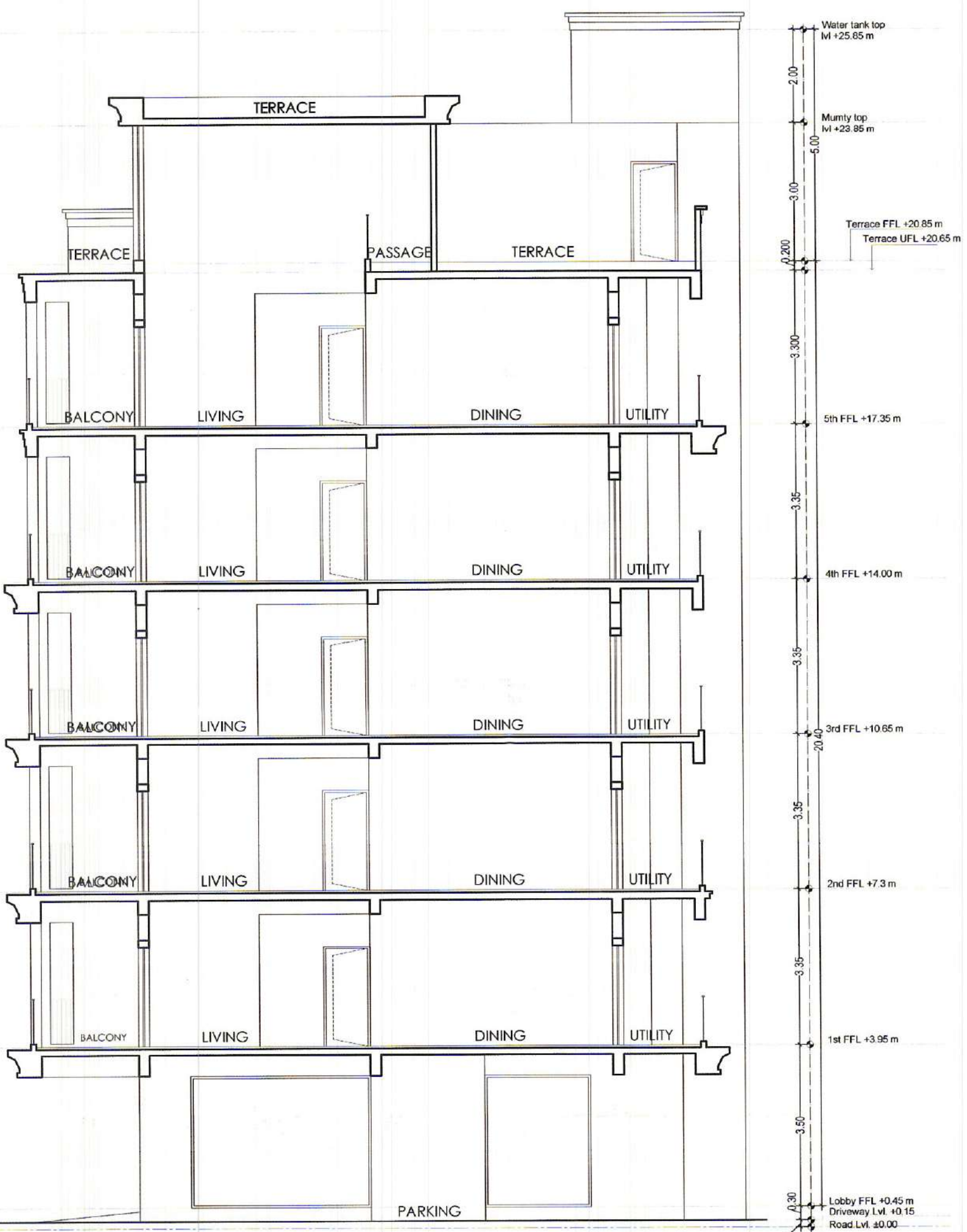
SECTION - YY
