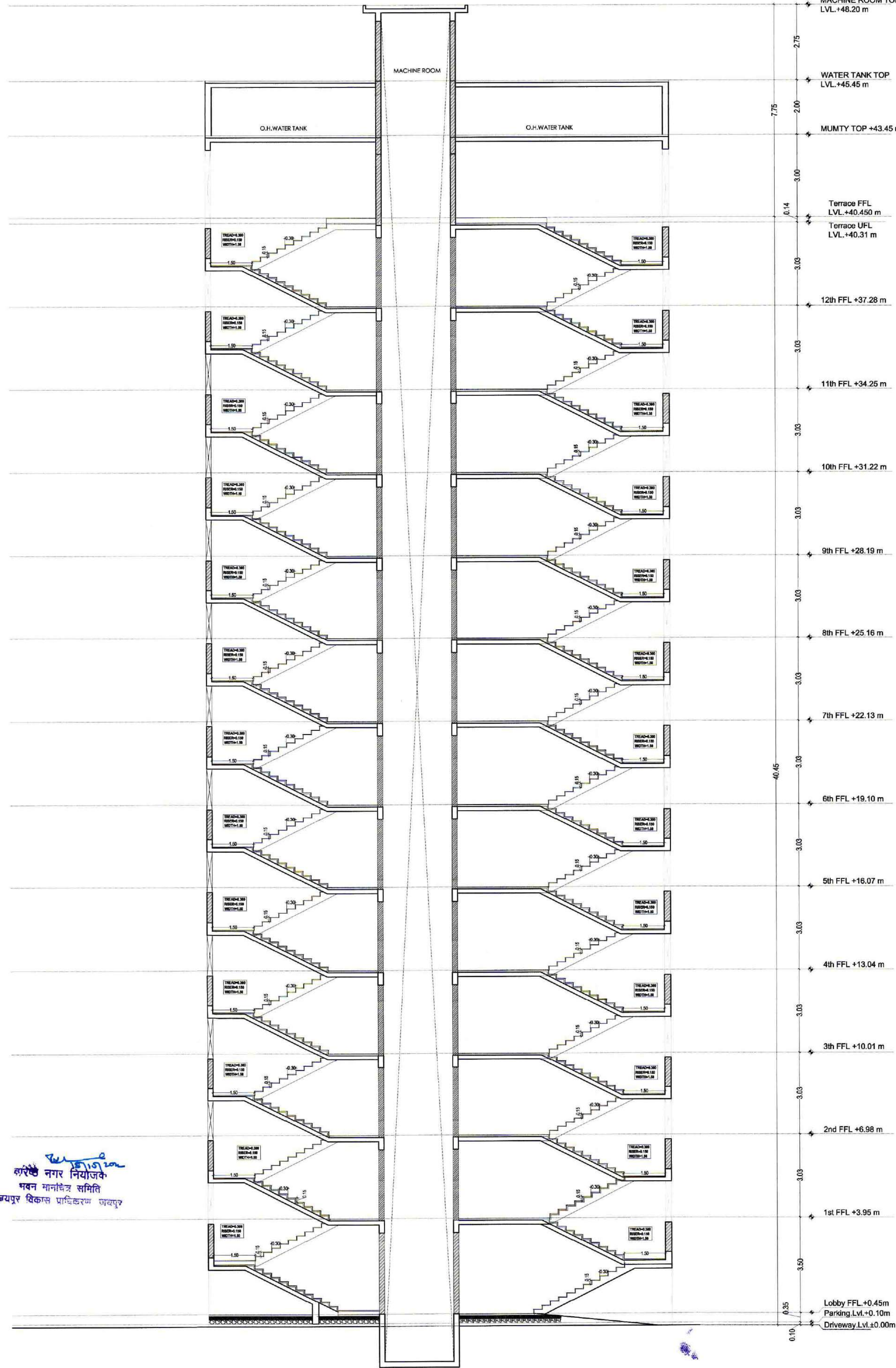
SECTION @_X
